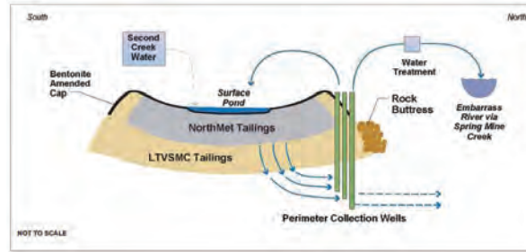
Cross section of a version of the Polymet tailings basin with seepage capture and geotechnical stability features.
